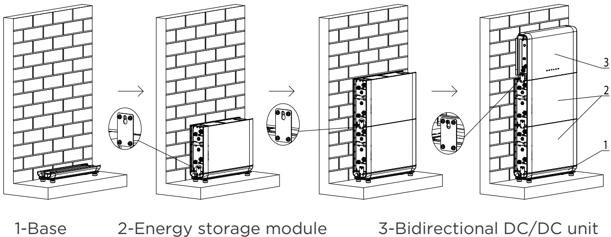
Figure.3-5 Installing the energy storage and bidirectional DC/DC unit diagram
